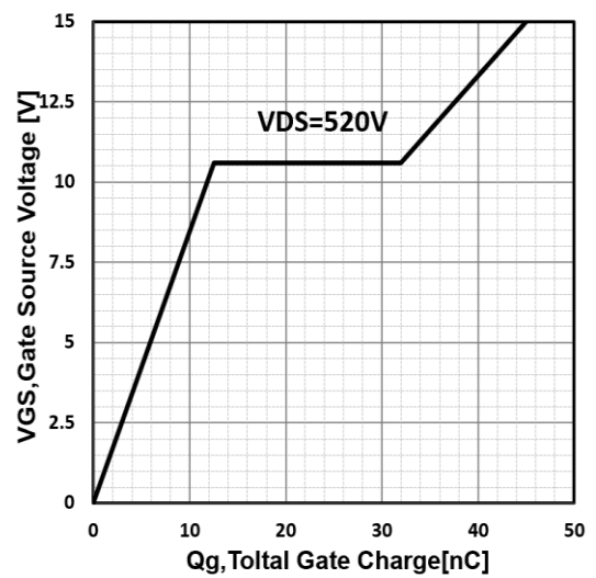
Figure 4. Typical gate charge VS. V_{GS} , V_{GS} , Gate Source Voltage, V_{DS}=520\text{V} , I_C=20\text{A}
