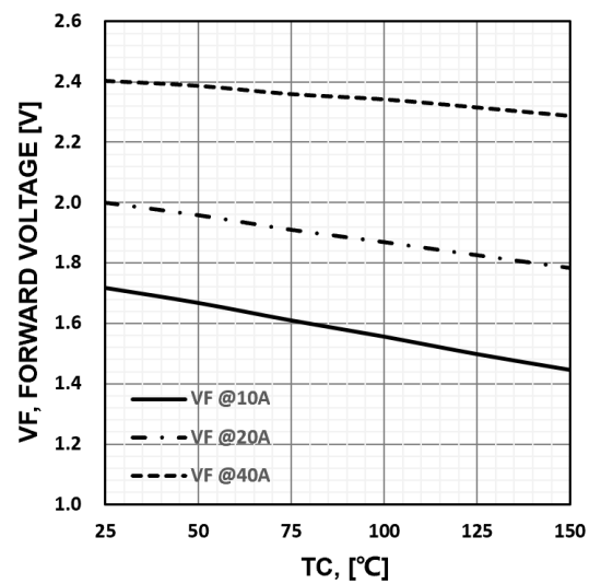
Figure 8. Typical forward voltage vs IF
