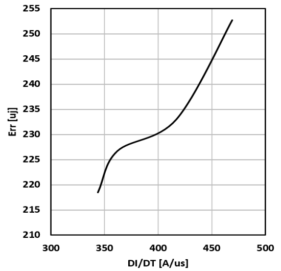
Figure 16. Typical diode Err vs di/dt Tc=25°C VCC=400V VGE=15V IF=20A
