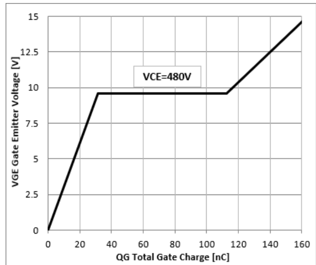
Figure 4: Typical Gate charge VS. V_{GE} , I_C=60\text{A}
