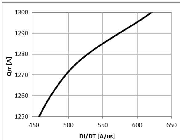
Figure 15: Typical Diode Qrr VS. DI/DT, TC=25°C VCC=400V, VGE=15V, IF=60A
