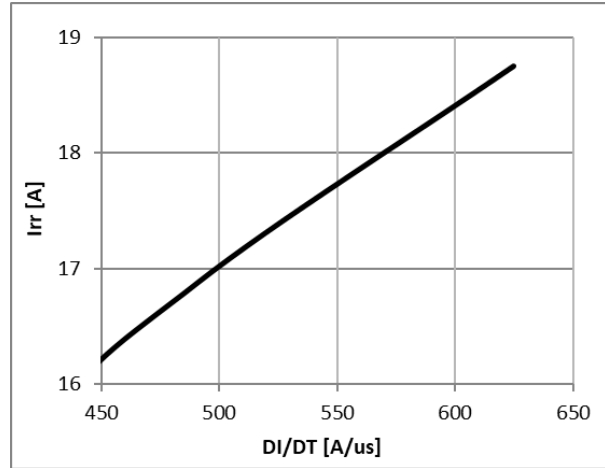
Figure 14: Typical Diode Irr VS. DI/DT, TC=25°C VCC=400V, VGE=15V, IF=60A
