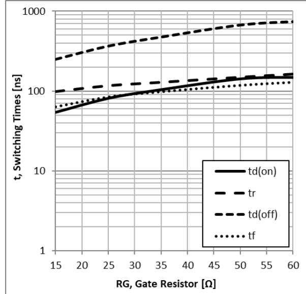
Figure 10: Typical Switching Time VS. RG, TC=25°C, L=200uH, VCE=400V, VGE=15V, IC=60A
