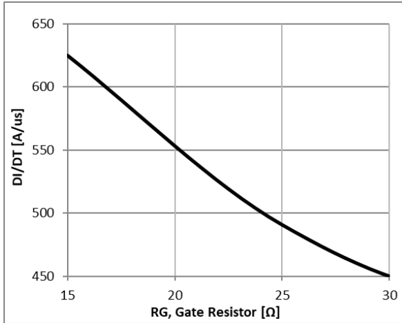
Figure 13: Typical Diode DI/DT VS. RG, TC=25°C VCC=400V, VGE=15V, IF=60A
