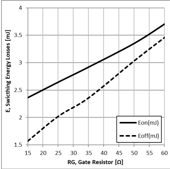
Figure 9: Typical Energy Loss VS. RG, TC=25°C, L=200uH, VCE=400V, VGE=15V, IC=60A
