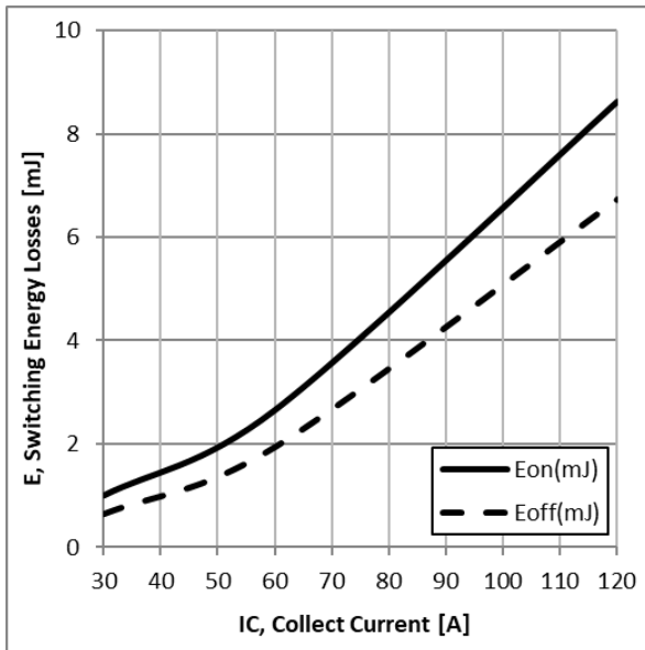
Figure 11: Typical Energy Loss VS. IC, TC=25°C, L=200uH, VCE=400V, VGE=15V, RG=25Ω
