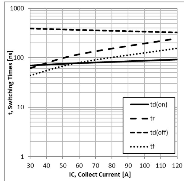
Figure 12: Typical Switching Time VS. IC, TC=25°C, L=200uH, VCE=400V, VGE=15V, RG=25Ω
