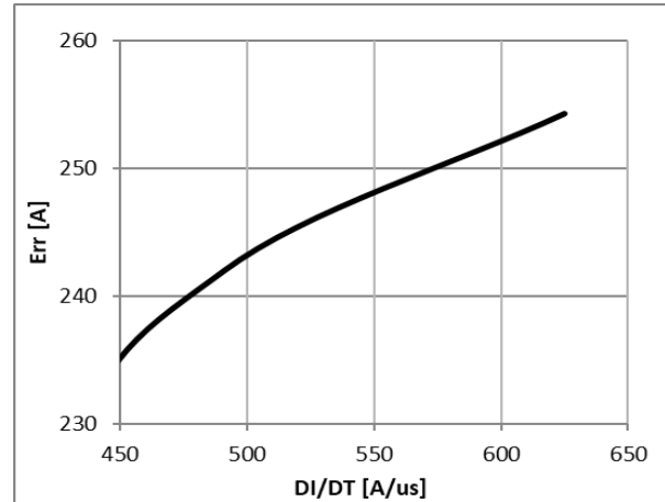
Figure 16: Typical Diode Err VS. DI/DT, TC=25°C VCC=400V, VGE=15V, IF=60A
