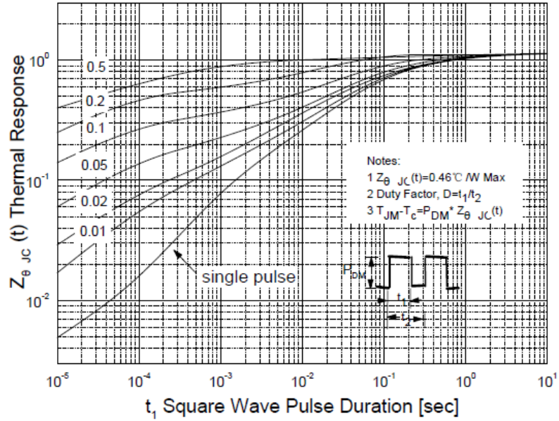
Figure 11-2. Transient Thermal Response Curve for JFAM20N60D
