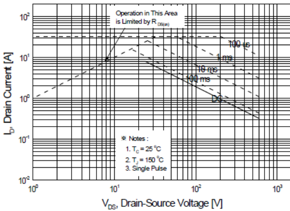
Figure 9-1. Maximum Safe Operating Area for JFPC7N60C
