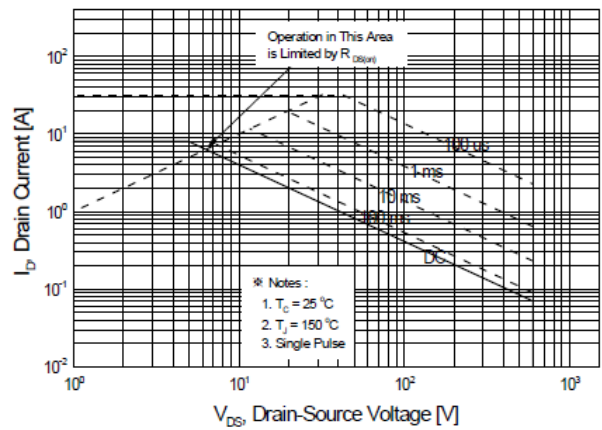
Figure 9-2. Maximum Safe Operating Area for JFFM7N60C
