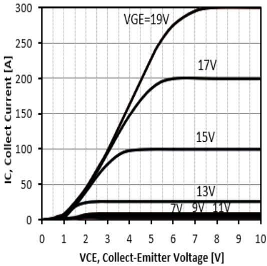
Figure 5: Typical IGBT Output Characteristics, TC=25°C;tp=300us
