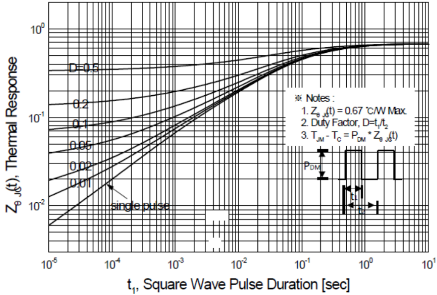
Figure 11-2. Transient Thermal Response Curve for JFPC10N65D
