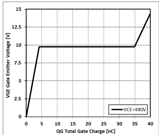
Figure 4: Typical Gate charge VS. V_{GE} , I_C=15\text{A}
