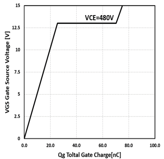
Figure 4: Typical gate charge VS. VGE, IC=40A
